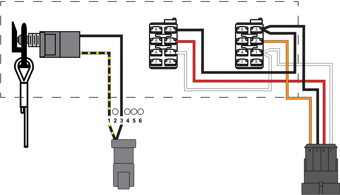
ICON II Start Stop Panel Dual Outboard Second Station
